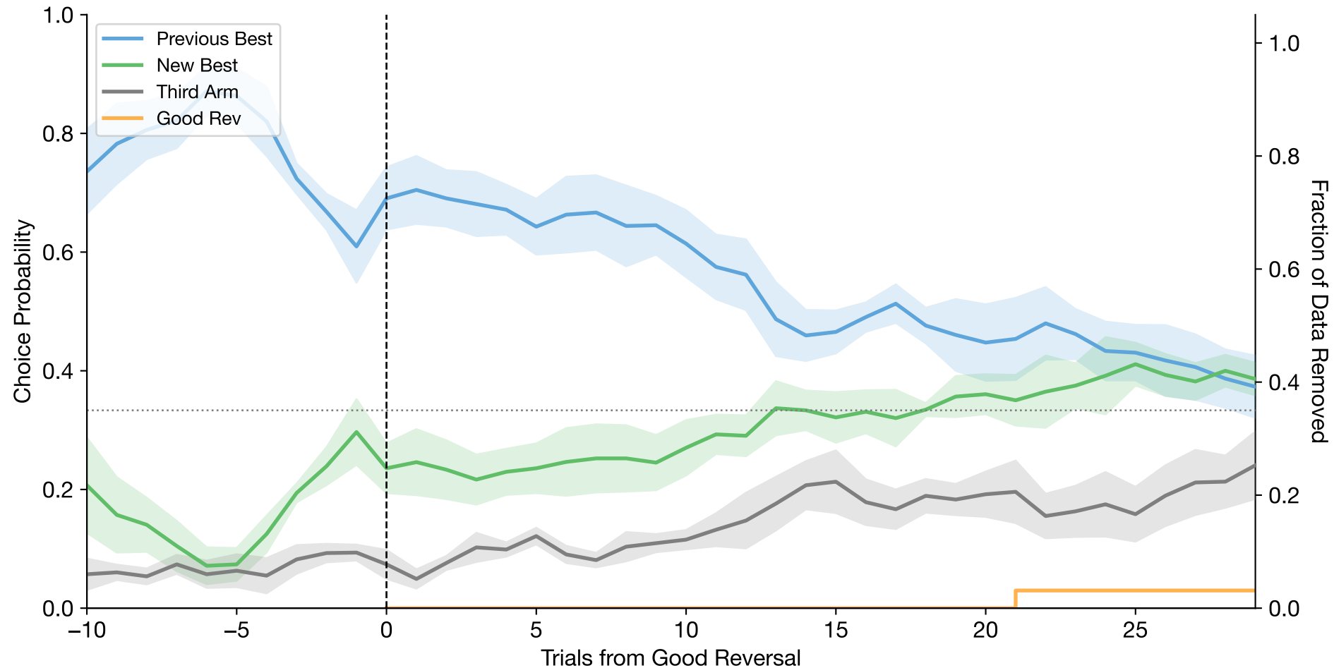
Good Reversal-Aligned Choices (mean \pm se across subjects | n=6 subjects, n=32 reversals)
